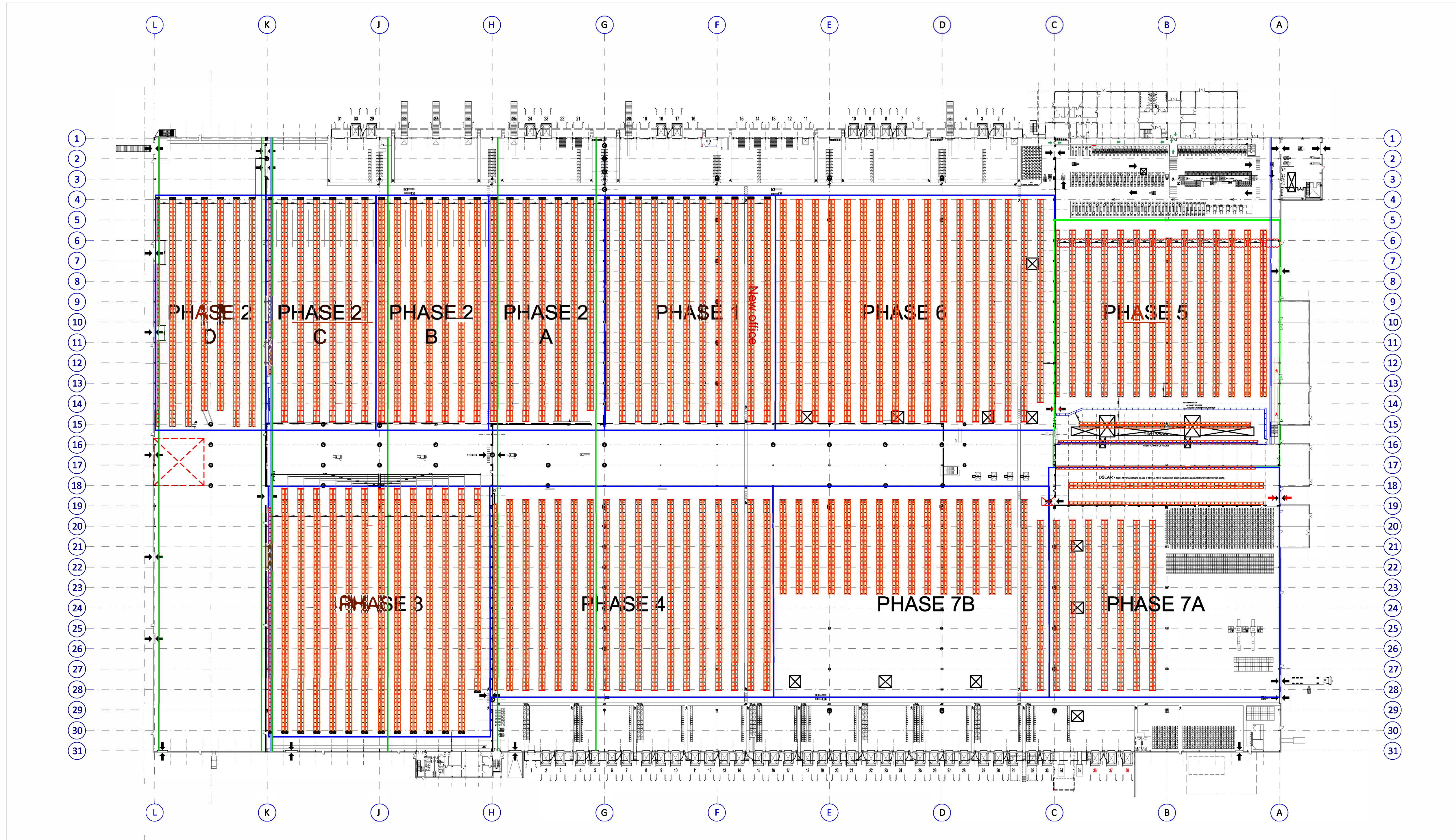
SITE RACKING PLAN Scale: 1:750 @A1
